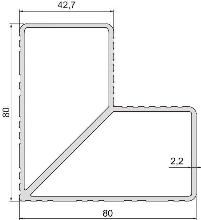
KOD-CODE KT-1427-00 TEORİK AĞIRLIK THEORETICAL WEIGHT 2,146 Kg/m
