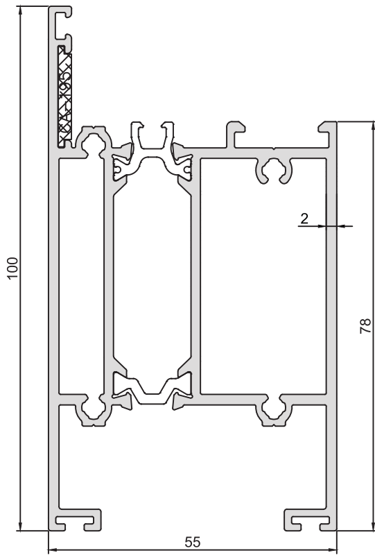
KOD-CODE AT-5551-20 TEORİK AĞIRLIK THEORETICAL WEIGHT 2,291 Kg/m
