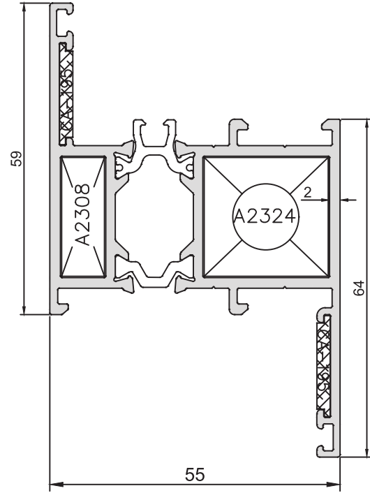
KOD-CODE AT-5517-20 TEORİK AĞIRLIK THEORETICAL WEIGHT 1,614 Kg/m
