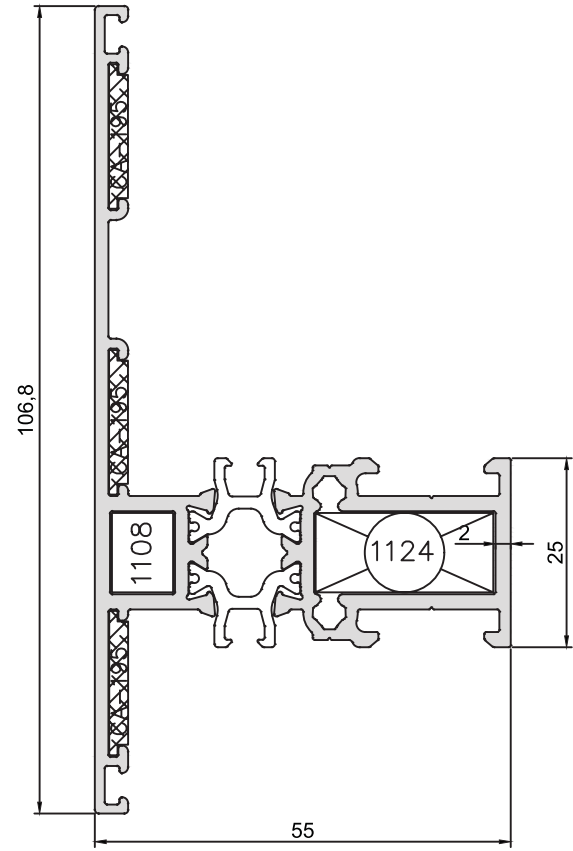
KOD-CODE AT-5528-20 TEORİK AĞIRLIK THEORETICAL WEIGHT 1,584 Kg/m
