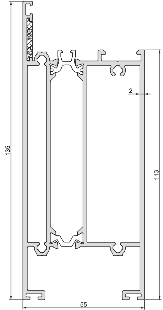
KOD-CODE AT-5552-20 TEORİK AĞIRLIK THEORETICAL WEIGHT 3,012 Kg/m
