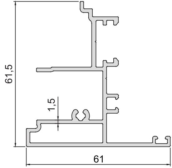
KOD-CODE AC-5561-15 TEORİK AĞIRLIK THEORETICAL WEIGHT 1,045 Kg/m
