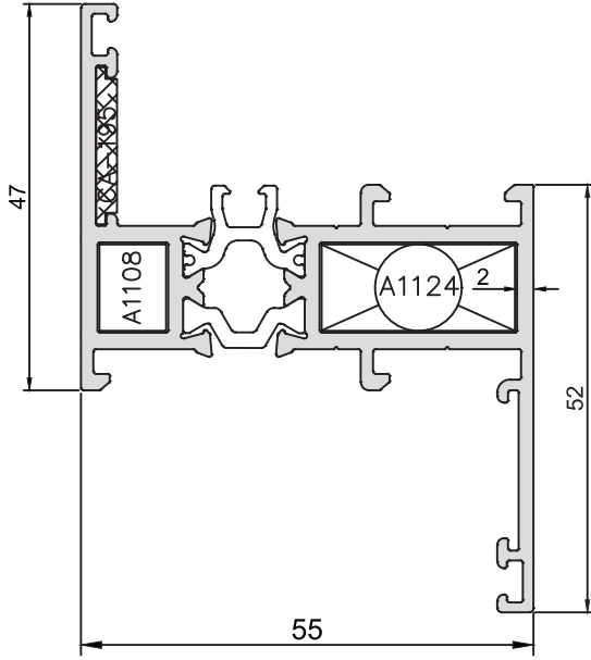
KOD-CODE AT-5516-20 TEORİK AĞIRLIK THEORETICAL WEIGHT 1,354 Kg/m
