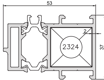
KOD-CODE AT-5568-20 TEORİK AĞIRLIK THEORETICAL WEIGHT 1,200 Kg/m
