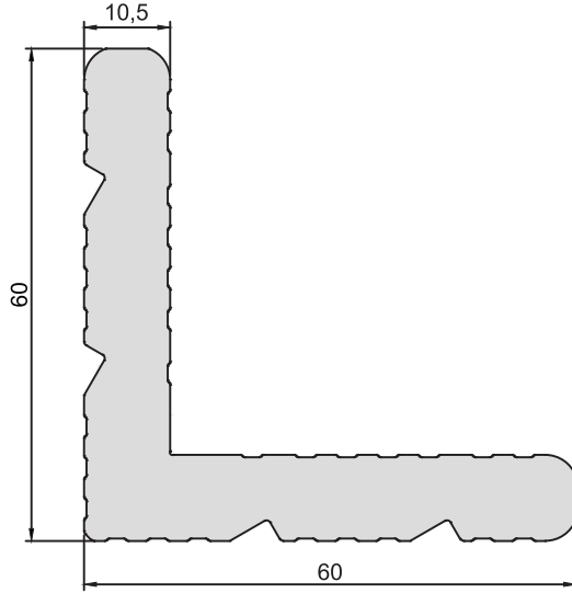
KOD-CODE KT-2105-00 TEORİK AĞIRLIK THEORETICAL WEIGHT 2,938 Kg/m
