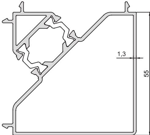
KOD-CODE AT-5565-13
