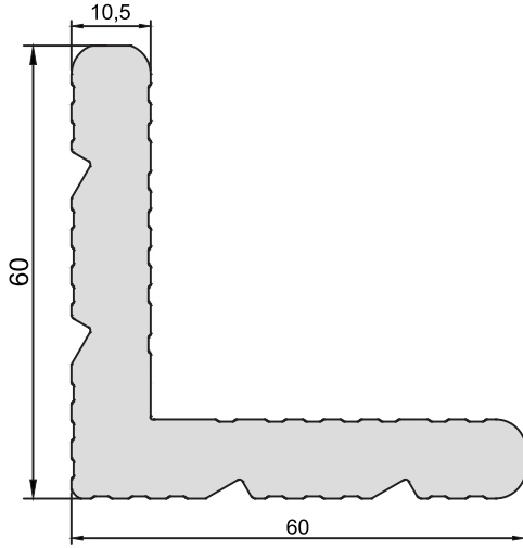
KOD-CODE KT-2105-00 TEORİK AĞIRLIK THEORETICAL WEIGHT 2,938 Kg/m
