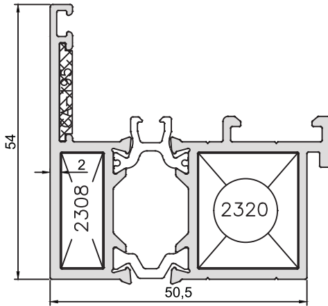
KOD-CODE AT-5563-20
