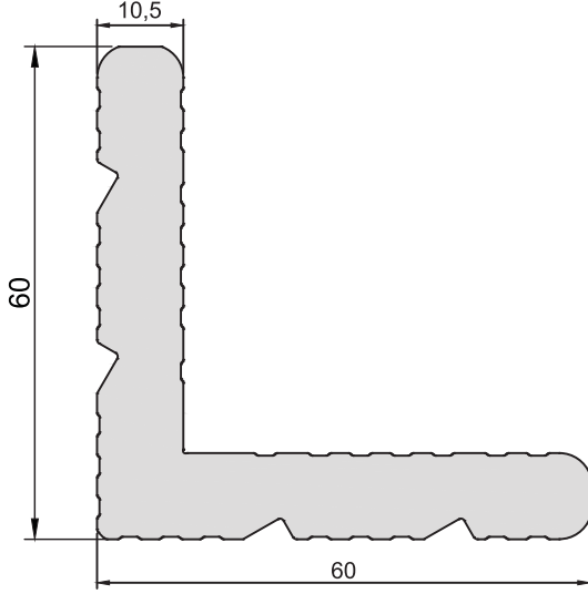
KOD-CODE TEORİK AĞIRLIK KT-2105-00 THEORETICAL WEIGHT 2,938 Kg/m
