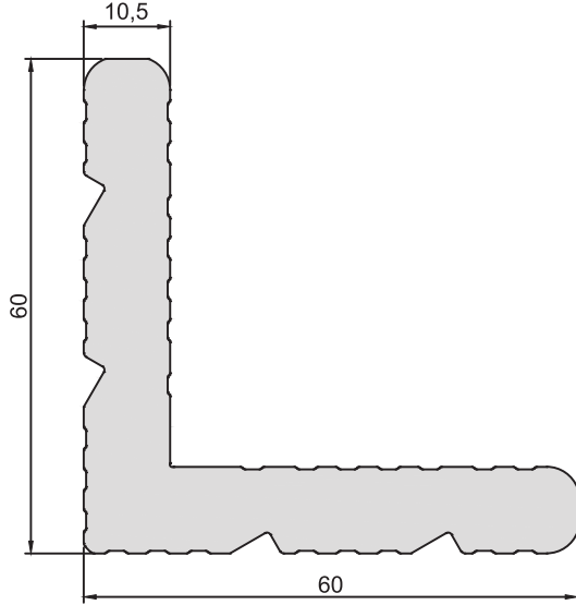
KOD-CODE TEORİK AĞIRLIK KT-2105-00 THEORETICAL WEIGHT 2,938 Kg/m
