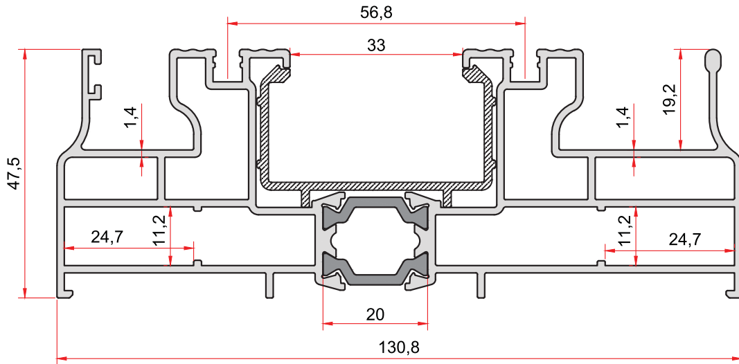
KOD-CODE TEORİK AĞIRLIK THEORETICAL WEIGHT ASS-4511-14 2,603 Kg/m
