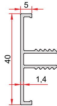
KOD-CODE TEORİK AĞIRLIK THEORETICAL WEIGHT AO-1042-14 0,286 Kg/m
