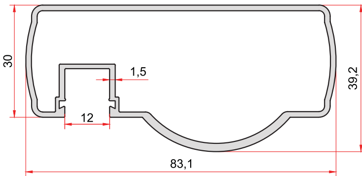
KOD-CODE TEORİK AĞIRLIK THEORETICAL WEIGHT 1907 1,053 Kg/m
