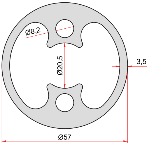
KOD-CODE TEORİK AĞIRLIK THEORETICAL WEIGHT 1865 2,843 Kg/m
