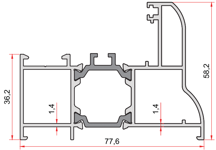
KOD-CODE TEORİK AĞIRLIK İD-102-14 THEORETICAL WEIGHT 1,506 Kg/m
