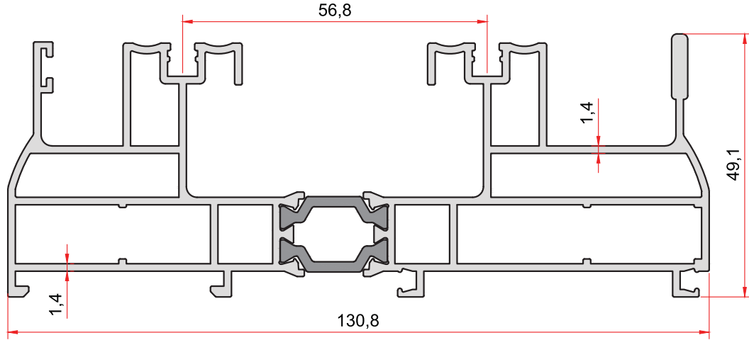
KOD-CODE TEORİK AĞIRLIK SS-102-14 THEORETICAL WEIGHT 2,678 Kg/m
