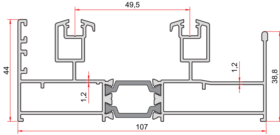
KOD-CODE TEORİK AĞIRLIK THEORETICAL WEIGHT MD-103-12 1,825 Kg/m
