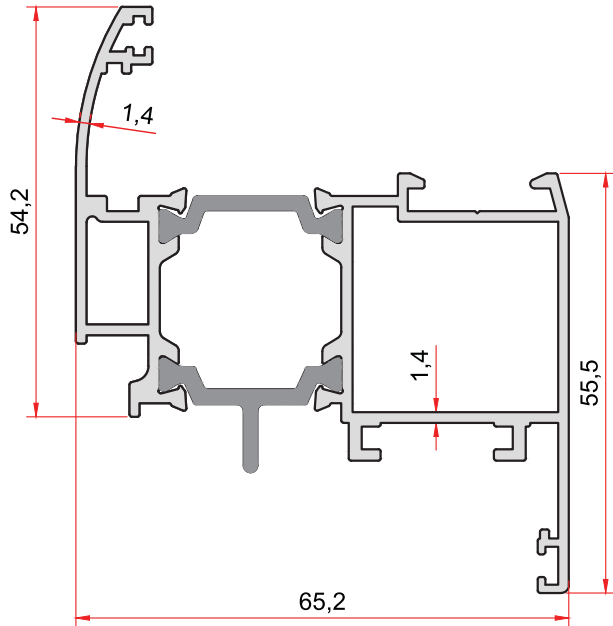
KOD-CODE TEORİK AĞIRLIK İD-402-14 THEORETICAL WEIGHT 1,457 Kg/m
