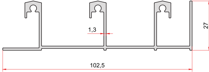
KOD-CODE TEORİK AĞIRLIK THEORETICAL WEIGHT 7032 1,000 Kg/m
