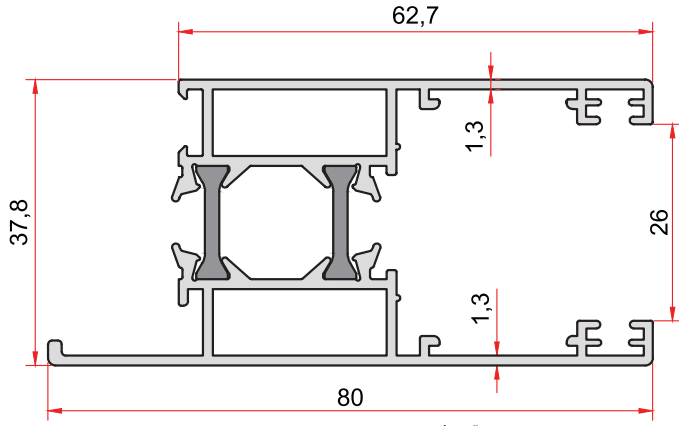
KOD-CODE TEORİK AĞIRLIK SS-203-13 THEORETICAL WEIGHT 1,239 Kg/m
