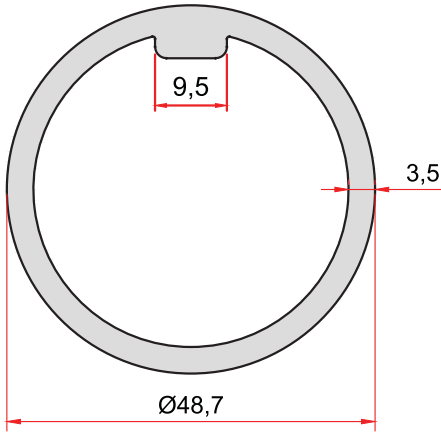
KOD-CODE TEORİK AĞIRLIK THEORETICAL WEIGHT 1854 1,426 Kg/m
