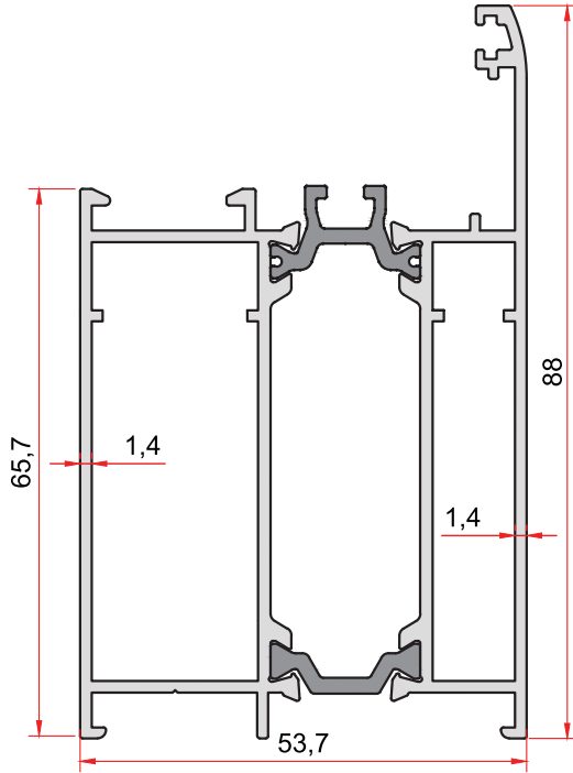
KOD-CODE TEORİK AĞIRLIK İD-103-14 THEORETICAL WEIGHT 1,699 Kg/m
