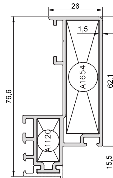
KOD-CODE AF-5066-15 TEORİK AĞIRLIK THEORETICAL WEIGHT 1,107 Kg/m
